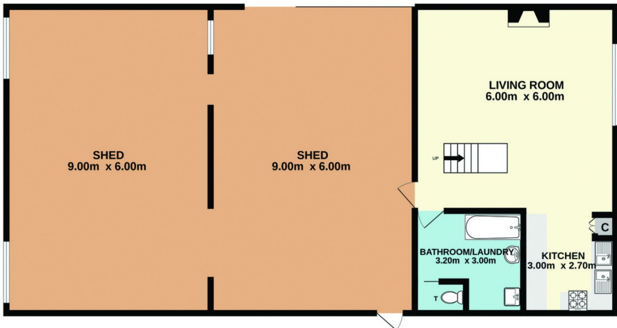
GROUND FLOOR 160.4 sq.m. approx.
